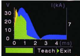
Weld Monitor
