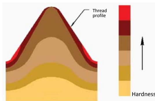
Rolled Threads = Tough studs
